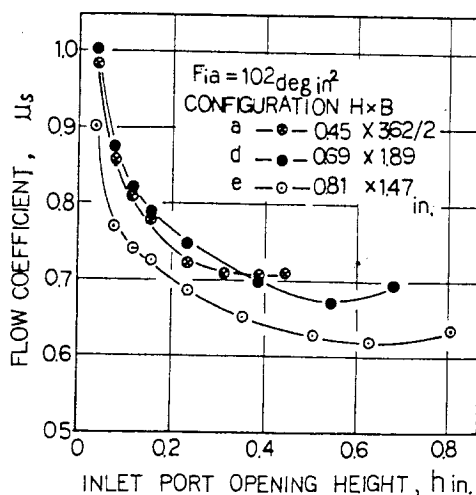
Fig. 37 - Relation between flow coefficient and inlet port opening height
