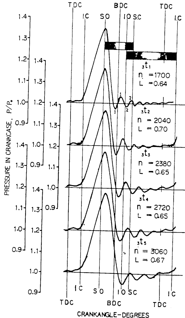
Fig. 15 - Crankcase indicator diagrams, case of 165T_3
