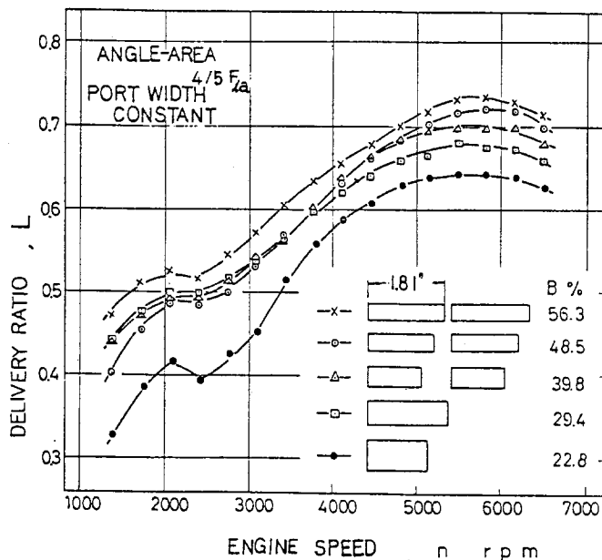
Fig. 26 (d) - Relation between delivery ratio and engine speed
