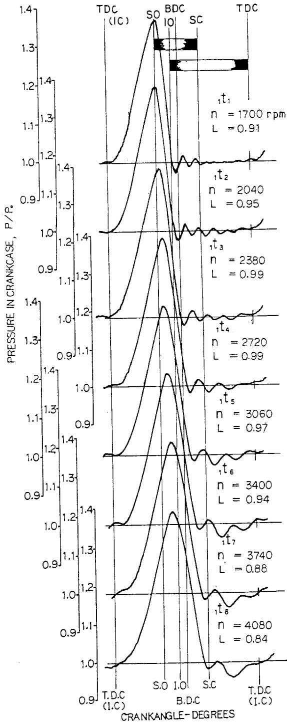
Fig. 12 - Crankcase indicator diagrams, case of 165T_1
