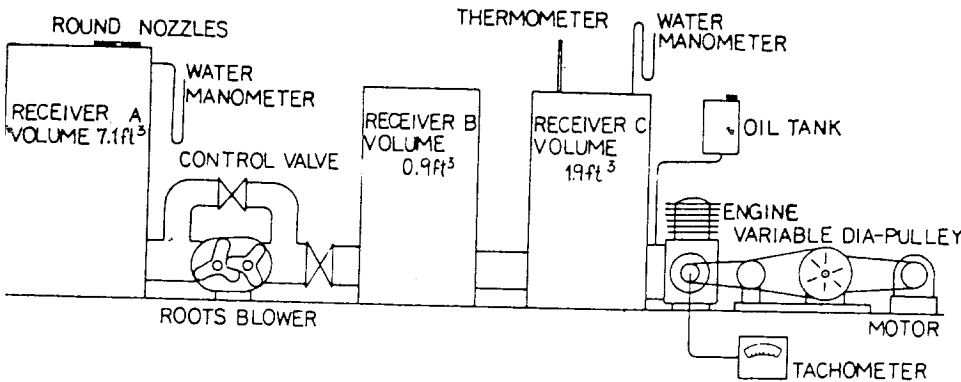
Fig. 1 - Test equipment used
