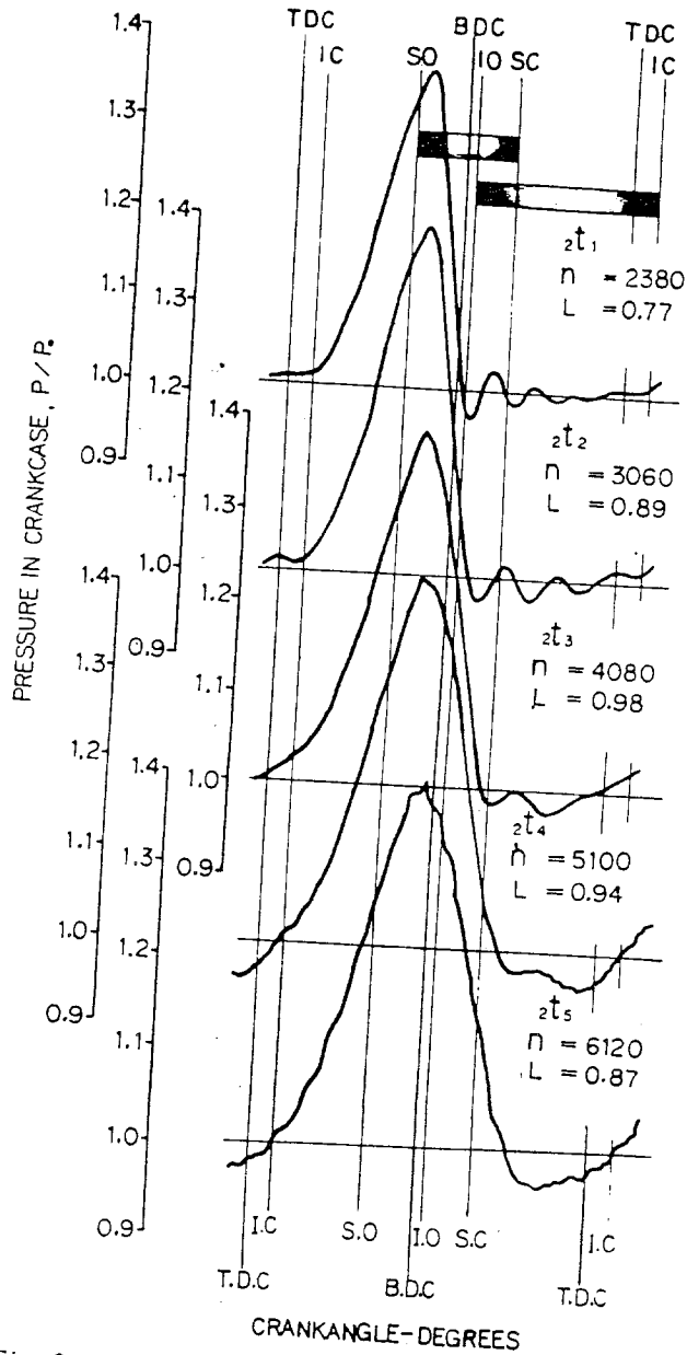
Fig. 9 - Crankcase indicator diagrams, case of 165 T_2
