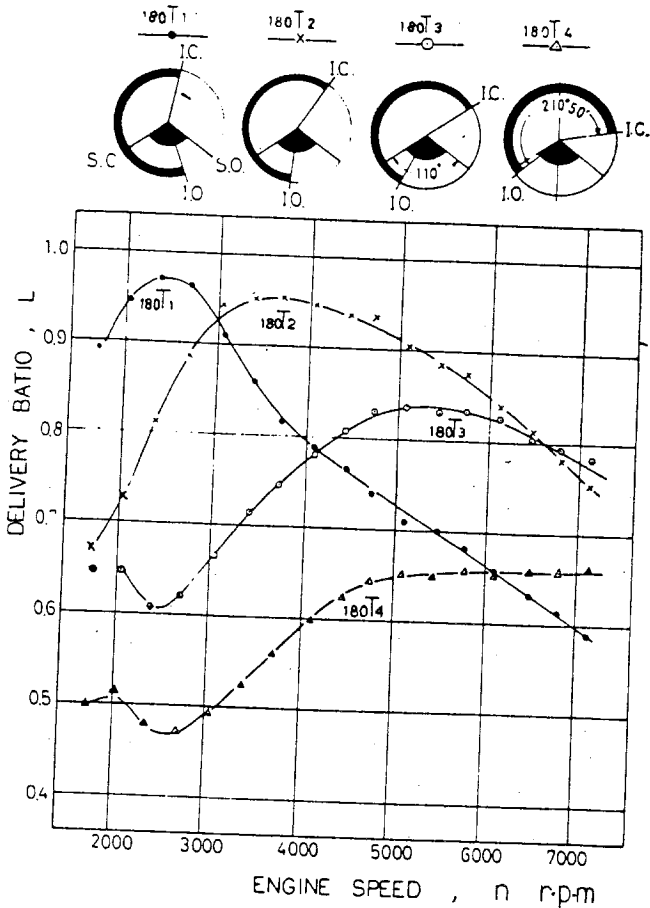
Fig. 4 (g) - Relation between delivery ratio and engine speed, 180 deg valve cut-angle
