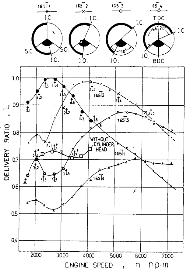
Fig. 4 (f) Relation between delivery ratio and engine speed, 165 deg valve cut-angle. Notations 1^1-7^1 2^1-5^1 3^1-5^1 , 3^1-3^1 correspond to each indicator diagram in Figs. 9, and 12-16
