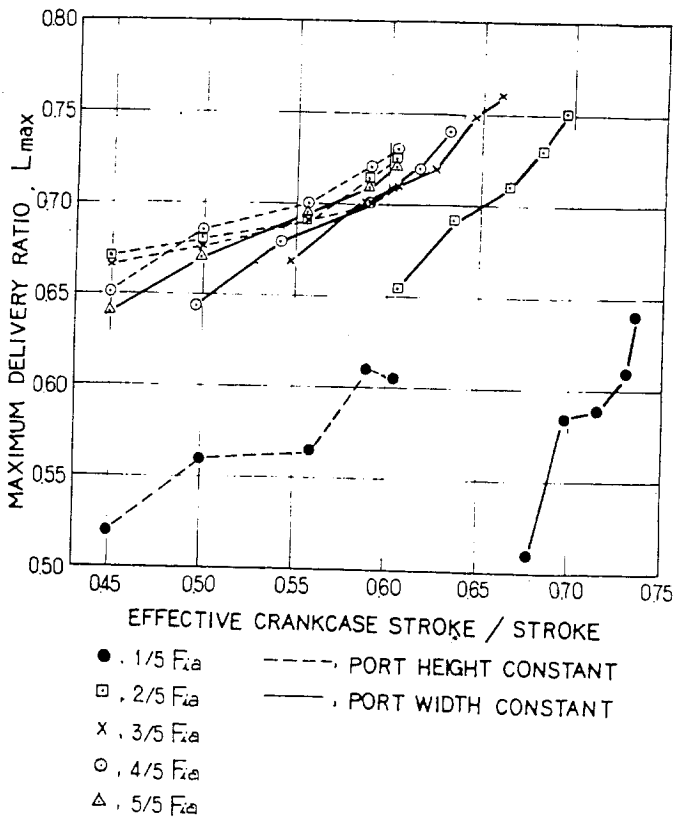
Fig. 29 - Relation between maximum delivery ratio and effective crankcase stroke. Dashed lines - when port width is changed at constant angle area. solid lines - when port height is changed at constant angle area
