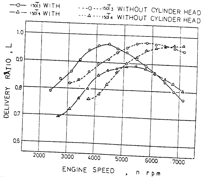
Fig. 18 - Relation between delivery ratio and engine speed, 150 deg valve cut-angle. Comparison of delivery ratio curves with and without cylinder head
