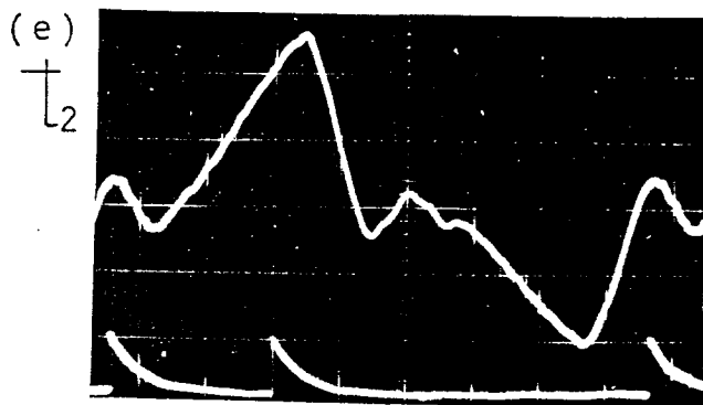
Fig. 26 (e) - Representative crankcase indicator diagram
