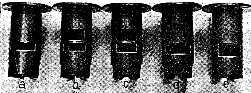
Fig. 21 - Cylinder liners having different inlet ports of constant angle area F_{ia} = 102 \text{ deg-in.}^2
