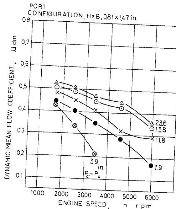
Fig. 38 (c) - Relation between flow coefficient and engine speed
