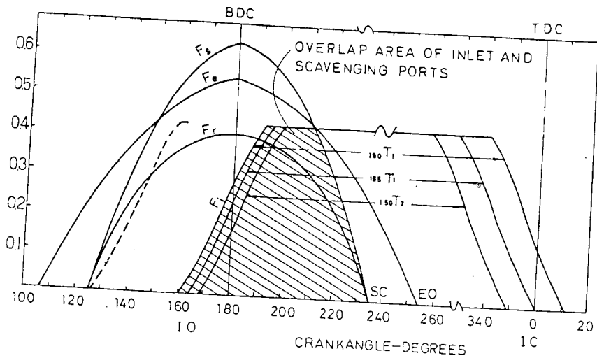
Fig. 10 - Relation between uncovered port area and crank angle
