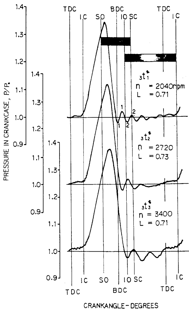
Fig. 16 - Crankcase indicator diagrams, case of T_{165} (without cylinder head)
