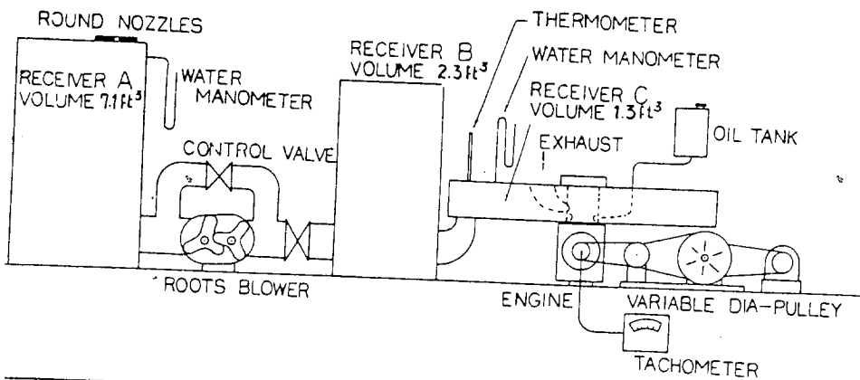
Fig. 19 - Test equipment used
