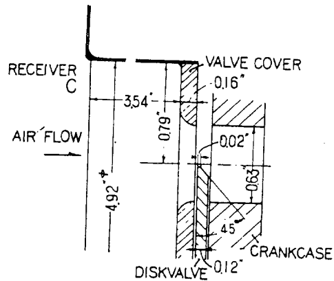
Fig. 2 - Inlet port in detail
