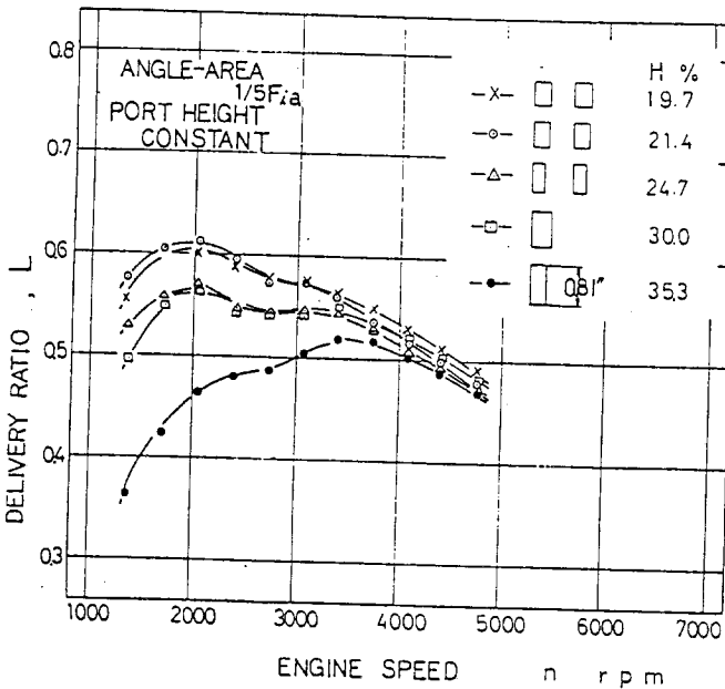
Fig. 27 (a) - Relation between delivery ratio and engine speed
