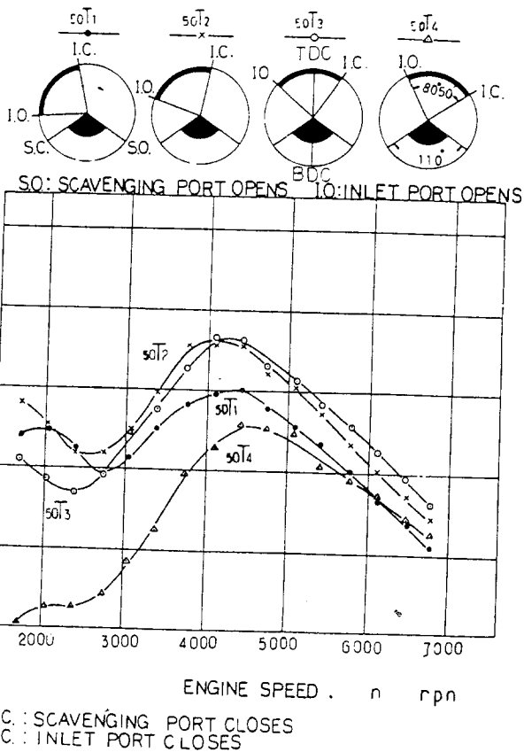
Fig. 4 (a) - Relation between delivery ratio and engine speed, 50 deg valve cut-angle
