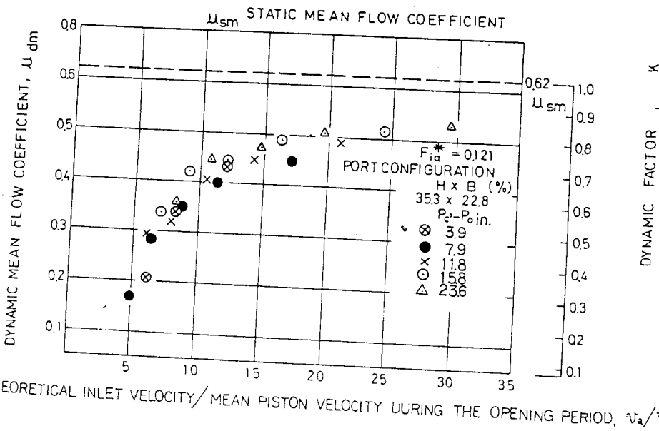
Fig. 40(c) - Relation between dynamic mean flow coefficient \mu_{dm} and V_a/\sqrt{V_p}
