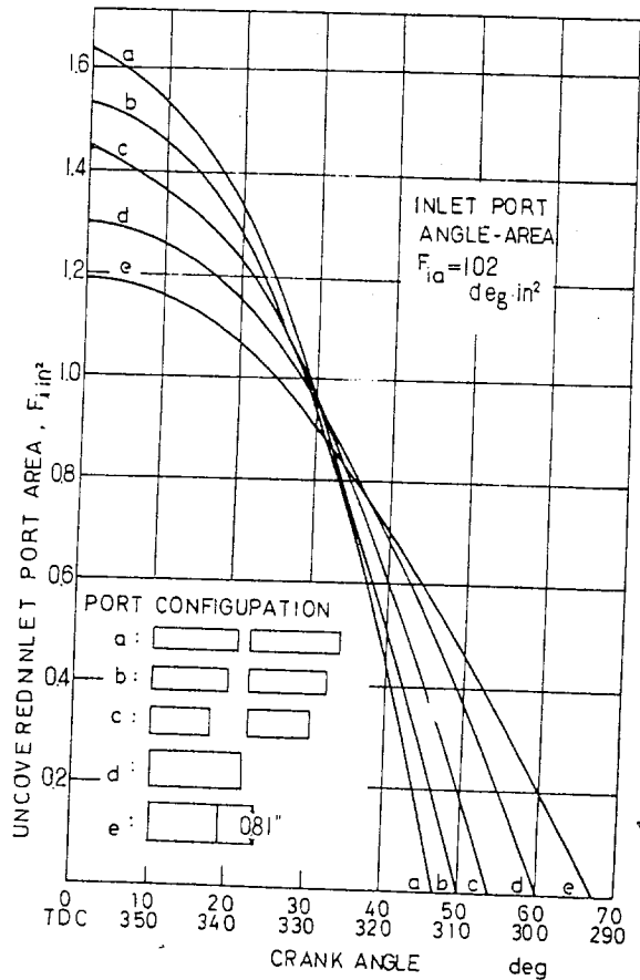
Fig. 23 - Relation between uncovered inlet port area and crank angle (all curves (a-e) have the same angle area)
